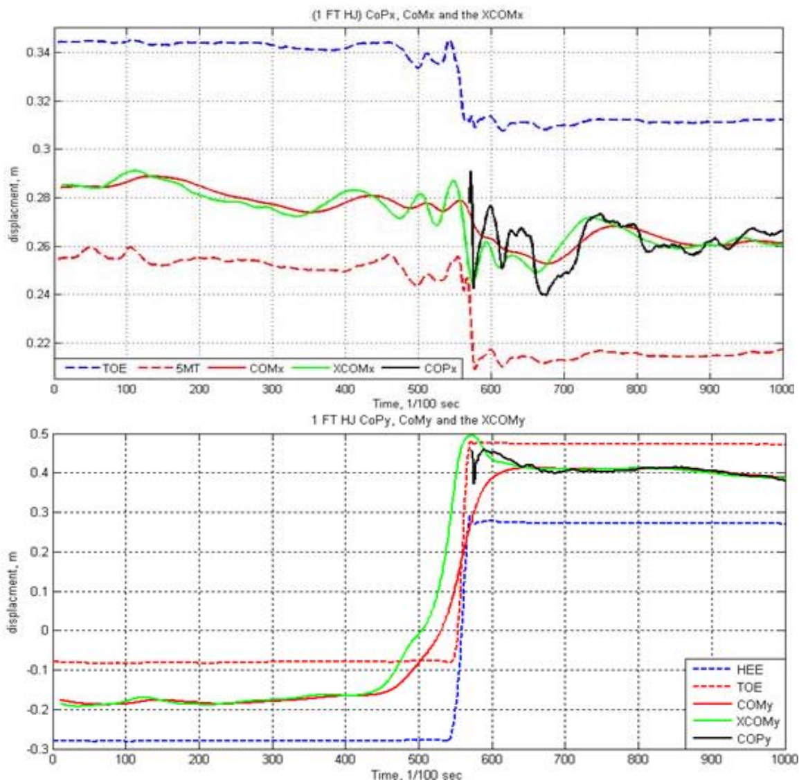
Fig. 10 Illustrates the variables CoP, CoM and XCoM in the ML (x) and the AP (y) directions are illustrated for dynamic balance (1-foot flat horizontal hop). (Units = m). Dashed lines indicate the boundaries of the Base of Support (BoS)
