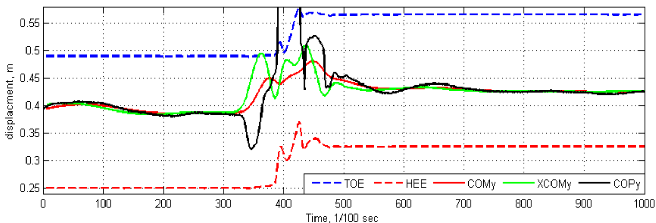
Fig. 6 The variables CoM, XCoM and CoP in the ML(x, upper) and the AP (y, lower) directions are illustrated for dynamic balance (2-feet flat vertical jump). (Units = m). Dashed lines indicate the boundaries of the Base of Support (BoS)
